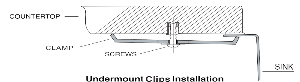
Undermount Clips Installation
