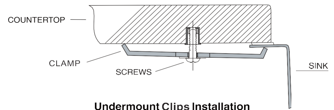
Undermount Clips Installation
